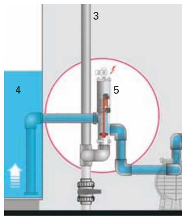
Overflow operation
